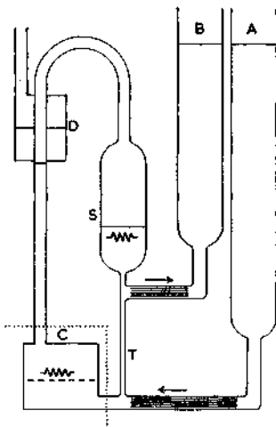
FIG. 9. Schematic diagram of dilution refrigerator. Dotted line separates cryostat C from recirculating mechanism. Dashed line in cryostat represents phase boundary, with concentrated He 3 solution on top. T is narrow capillary to flush dilute He 3 into still S. D is condenser. He 4 circulates from bath A through superleak, through T and out again through another superleak into bath B at higher temperature.
