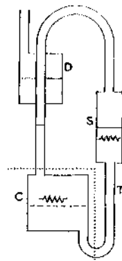
FIG. 10. Schematic diagram of dilution refrigerator. Cryostat C is like that in Fig. 9, but flow of dilute He 3 into still S is through wide tube T' and is non-turbulent. Motive force pulling He 3 round is pumping action exerted by condenser D.
