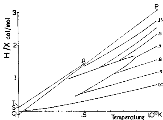
Fig. 7. Enthalpy per mole of He 3 as function of temperature for different concentrations. The curve for X=0 is not drawn. Q , S , and T are estimates of the heat of dilution at absolute zero.
